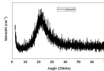
Figure 2 : DRX
